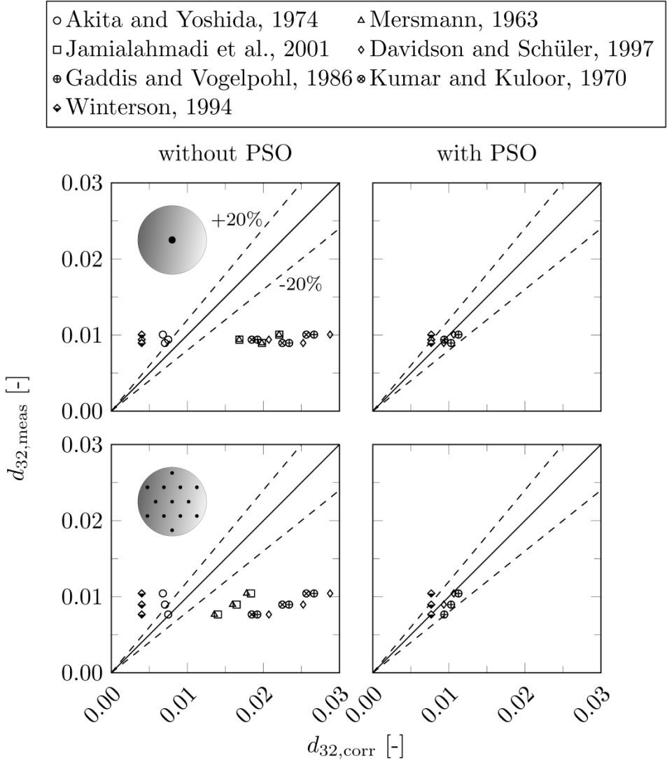
Figure 15: Comparison of the measured Sauter mean diameter with the one calculated using literature correlations.
