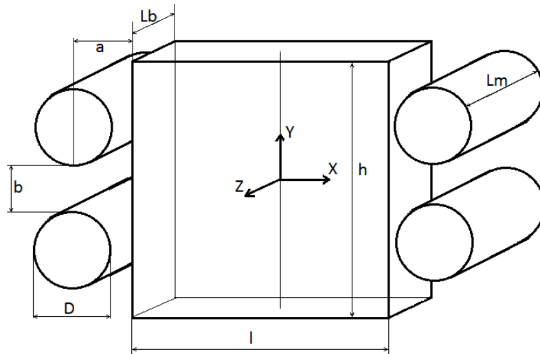
Fig. 1. Scheme of the permanent magnet stirrer.
